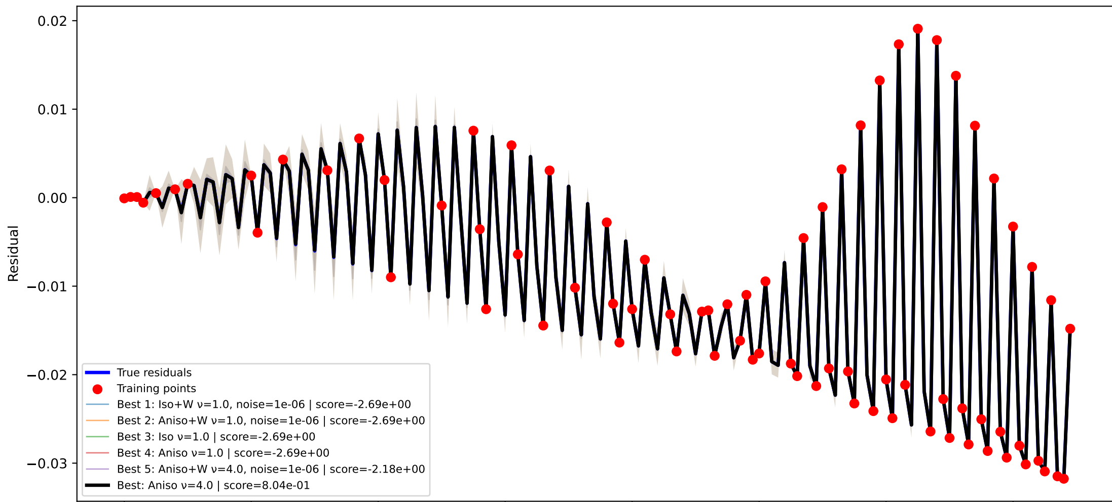
GPR kernel comparison node=20 RMSE=2.175e-05, train RMSE=9.255e-10
